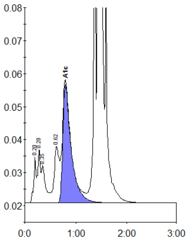
Peak table - ID: 10408662
